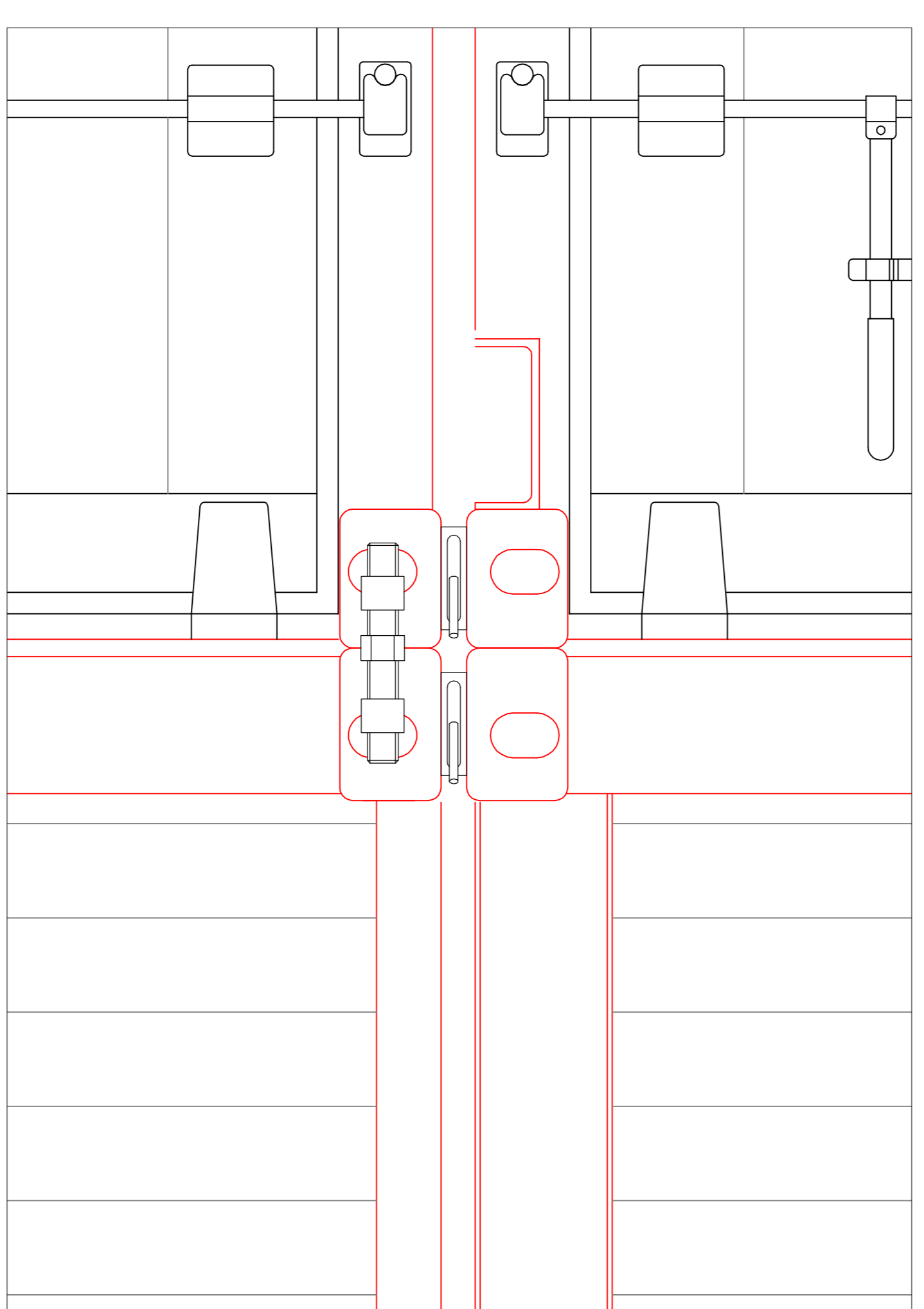
Four way connection
